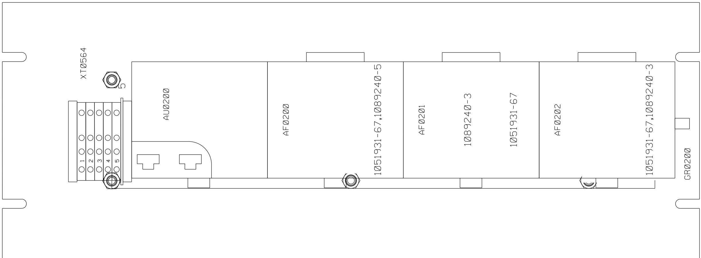
TYP. FOR XT0564
